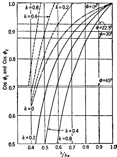
FIG. 4-10.—The dependence of \cos \phi_1 and \cos \phi_2 on \lambda/\lambda_\tau for various values of k in a double-strapped tube. The solid lines are \cos \phi_1 (symmetric modes); the broken lines are \cos \phi_2 (antisymmetric modes). For k = 0 the two sets of modes coincide.
